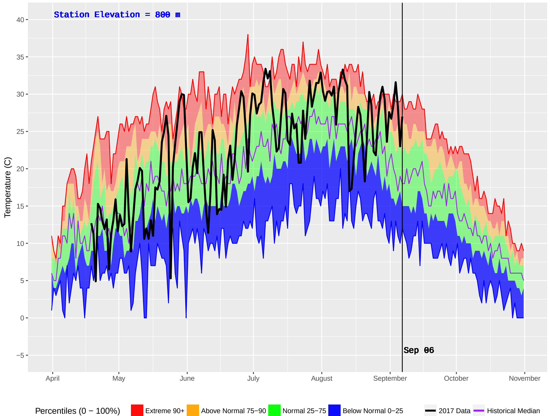
GOLD HILL (379) : Historical (1979–2016) and Current (2017) Noon Temperature
