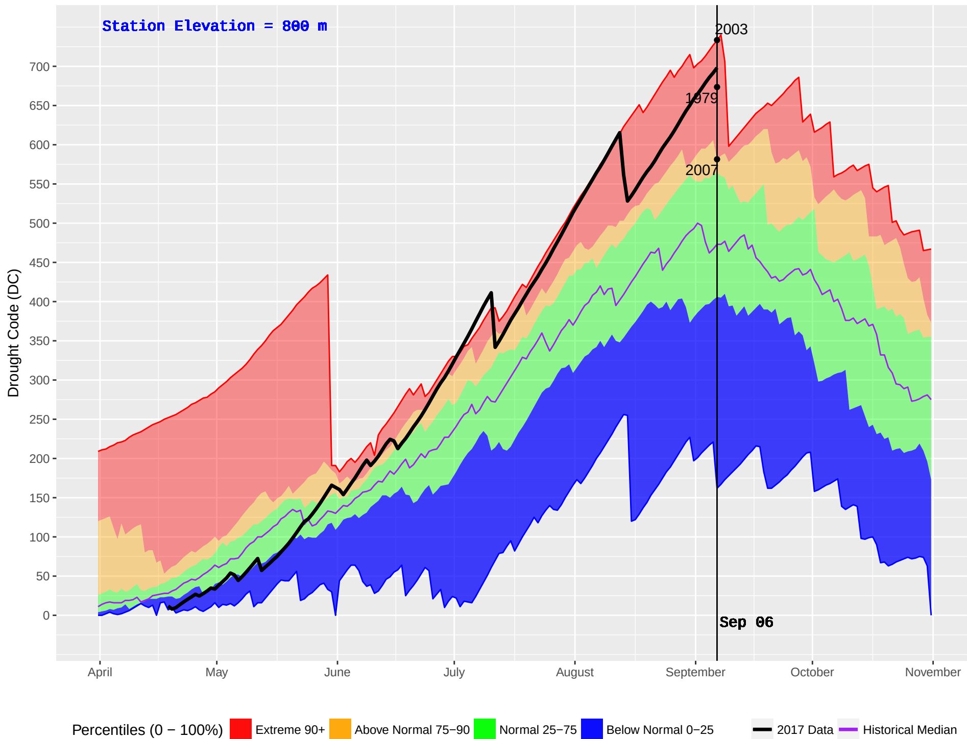
GOLD HILL (379) : Historical (1979–2016) and Current (2017) Noon Drought Code (DC)
