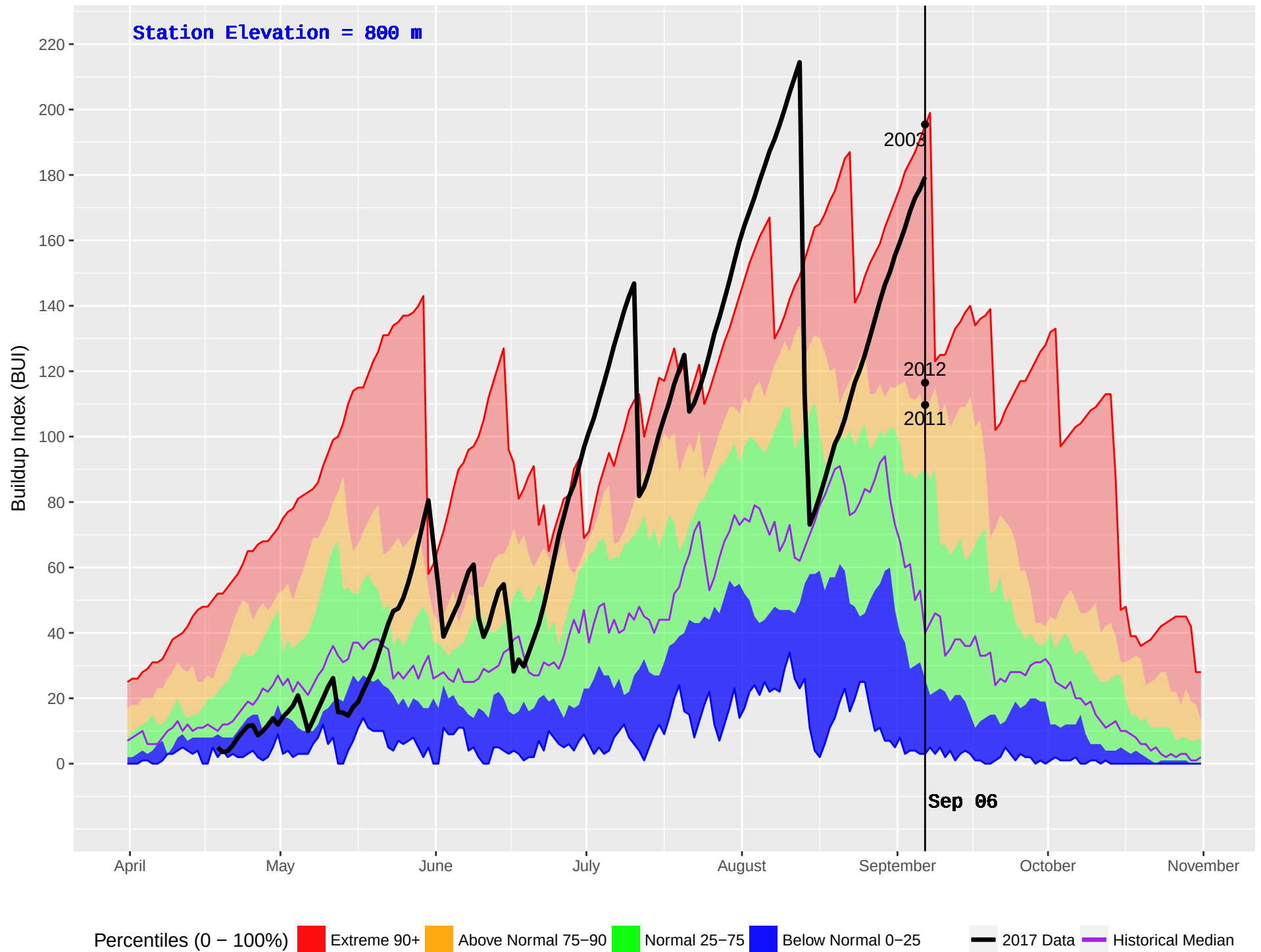
GOLD HILL (379) : Historical (1979–2016) and Current (2017) Noon Buildup Index (BUI)
